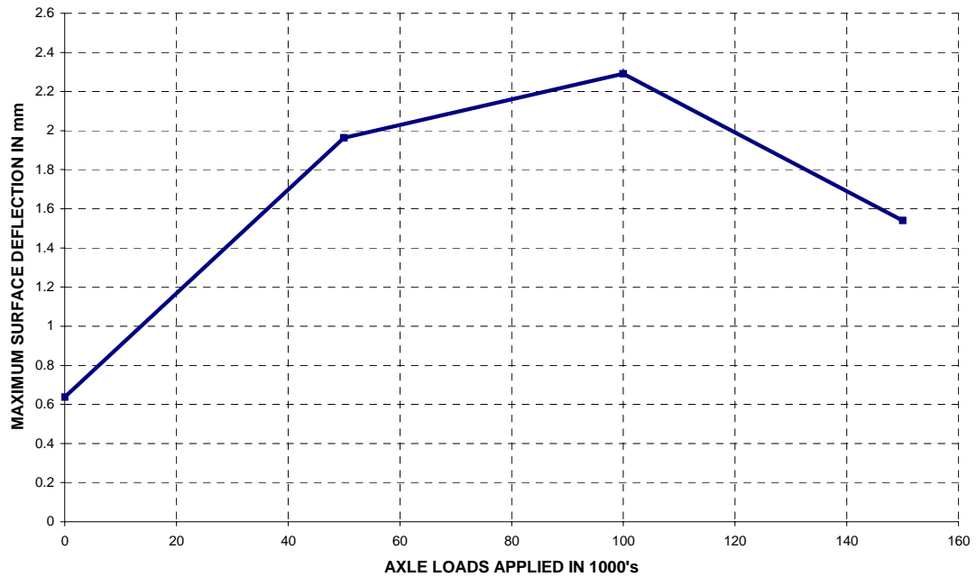
Figure B.1: Maximum Deflection at Slow Speed vs. Axle Load Application for Section 4B – 70 kN Axle Load
