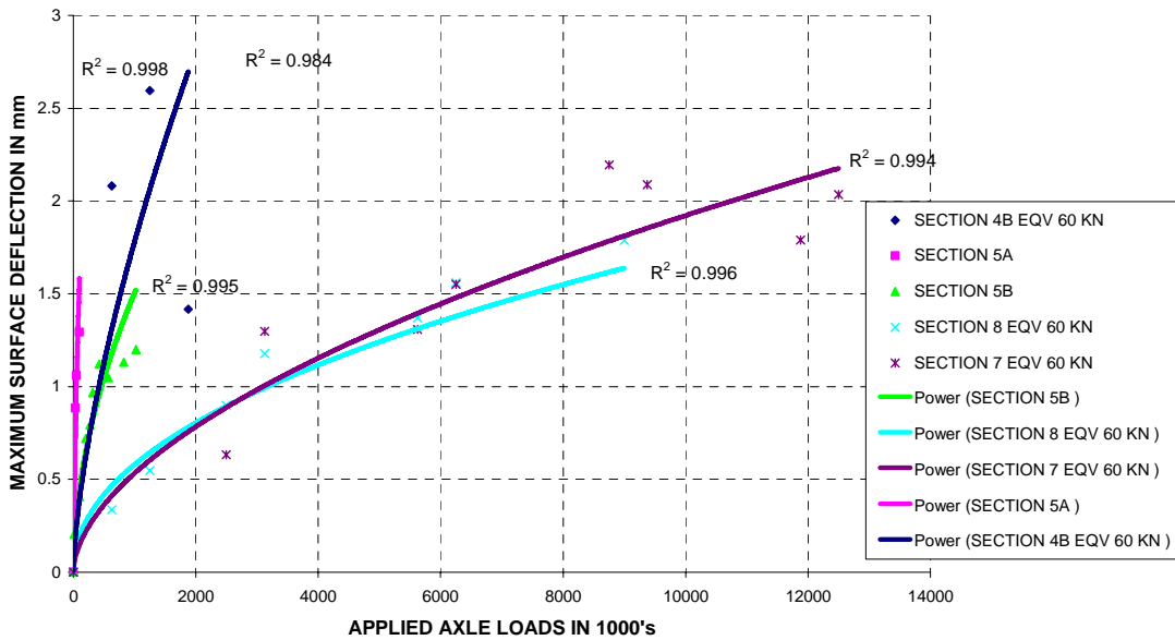
Figure B.6: Maximum Deflection Growth Trends with Equivalent 60 kN Axle Load Applications for Respective Test Sections
