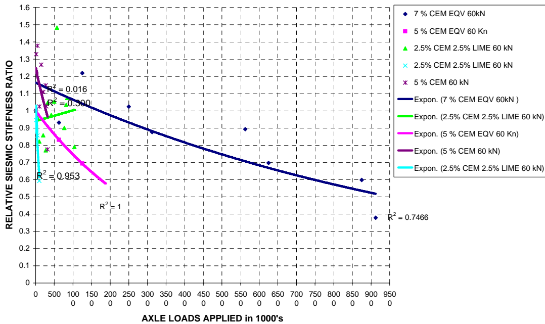
Figure C.4: Comparative Stiffness Performance Chart for Top of CTB in Transverse Direction for Equivalent 60 kN axle loads
