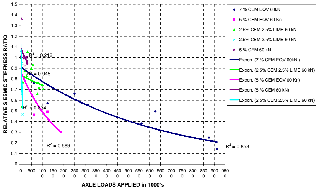
Figure C.6: Comparative Stiffness Performance Chart for Bottom of CTB in Transverse Direction for Equivalent 60 kN axle loads
