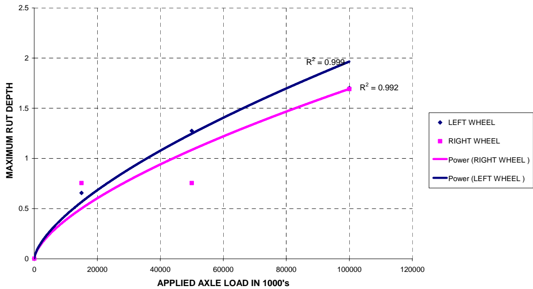
Figure D.6: Cumulative maximum rut depth for Test Section 5A
