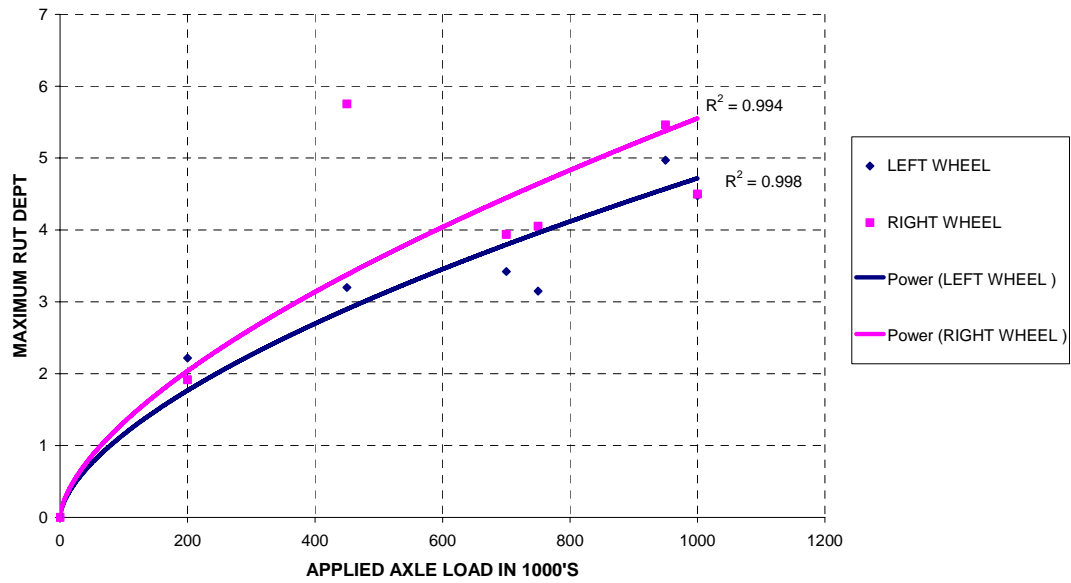
Figure D.12: Cumulative maximum rut depth for Test Section 7
