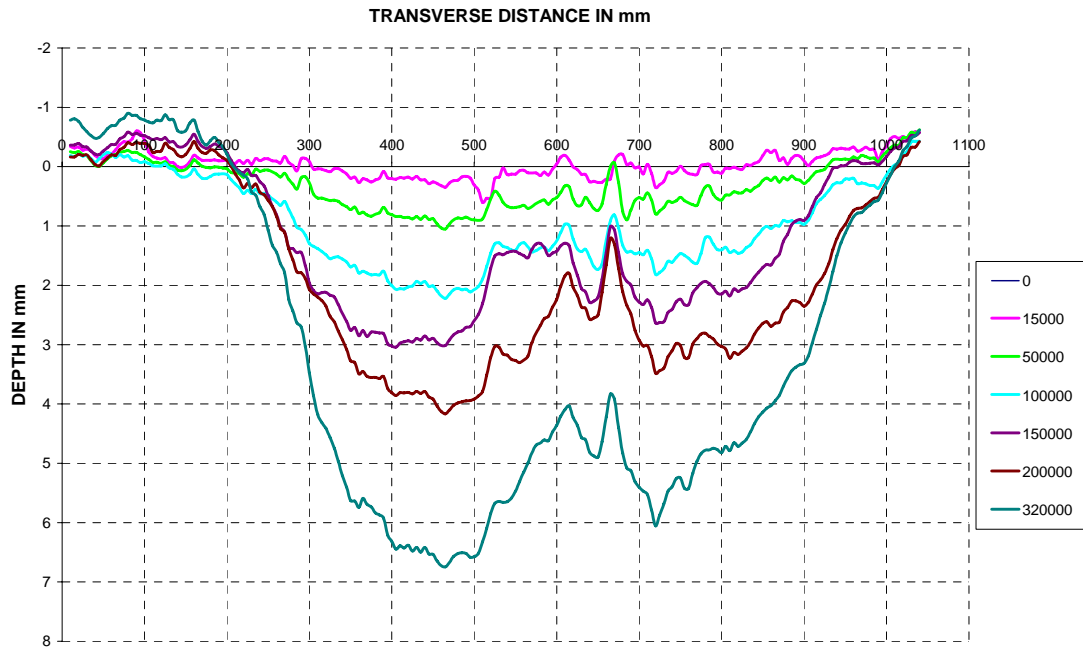
Figure D.1: Transverse rut profiles with load applications for Test Section 4A
