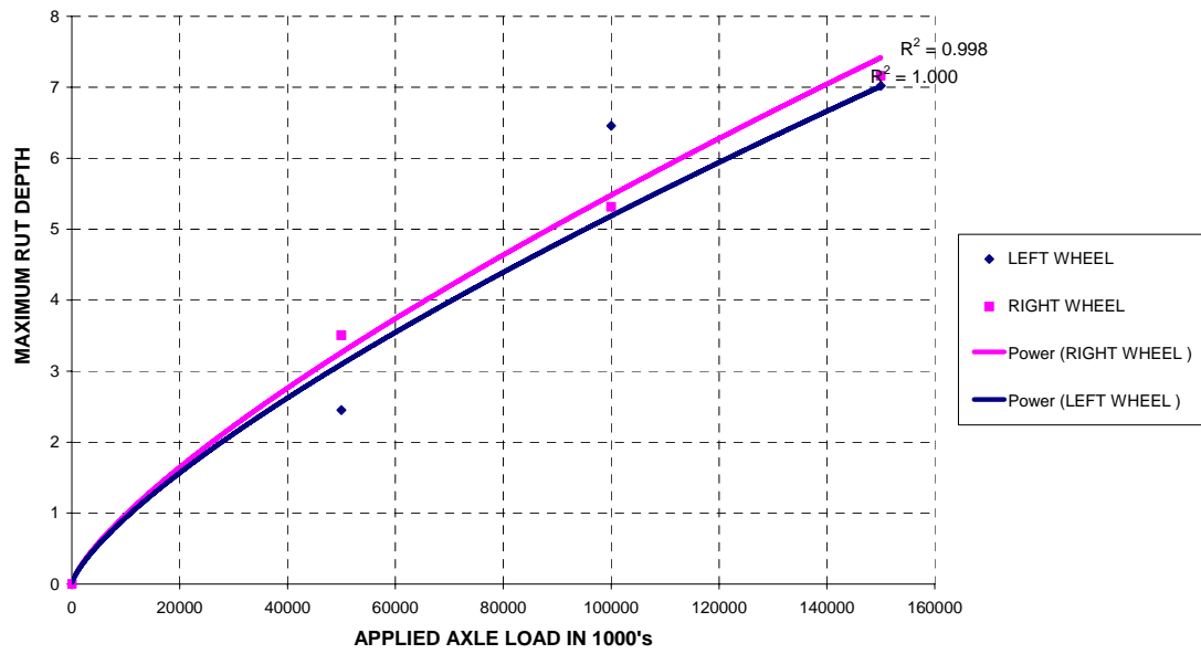
Figure D.4: Cumulative maximum rut depth for Test Section 4B
