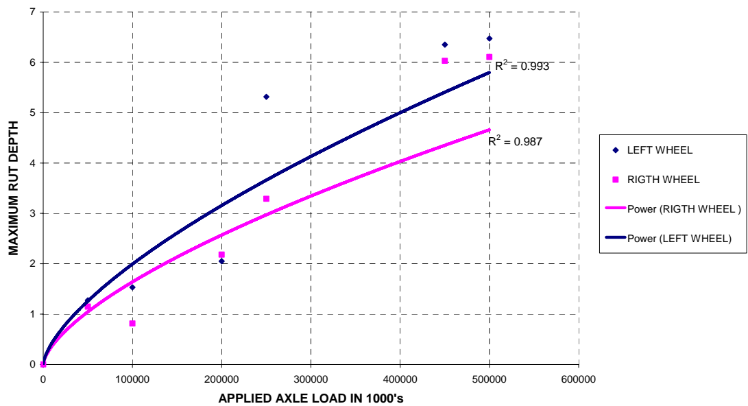
Figure D.10: Cumulative maximum rut depth for Test Section 8
