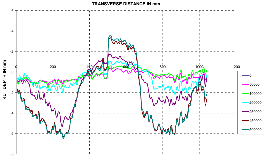
Figure D.9: Transverse rut profiles with load applications for Test Section 8
