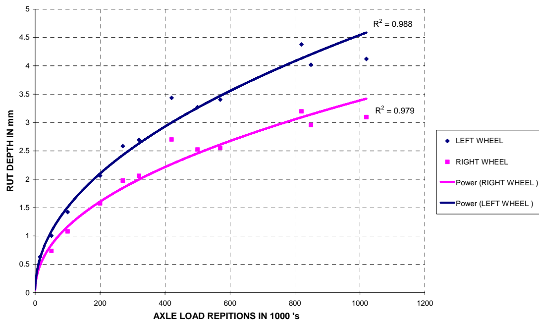
Figure D.8: Cumulative maximum rut depth for Test Section 5B
