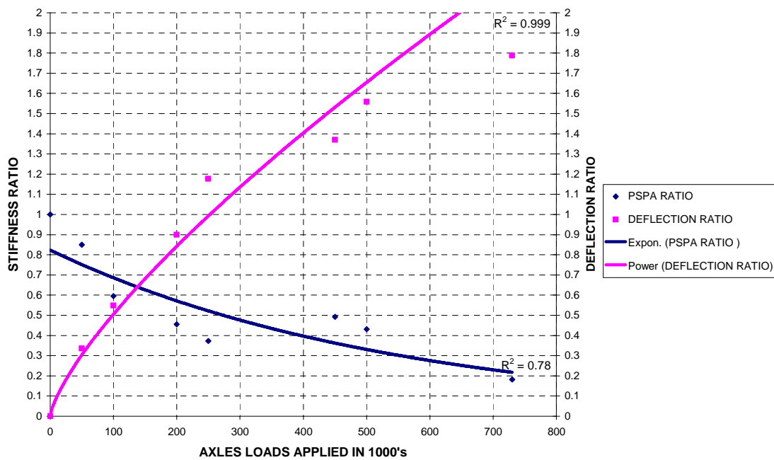
Figure K.6: Stiffness Deflectoin performacne trends of 7 % Cement stabilized Red base material under 70 kN axle loading
