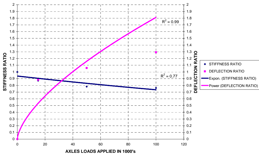
Figure K.4: Stiffness Deflection performance trends of 2.5 % Cement and 2.5 % Lime stabilized Red base material under 60 kN axle loading
